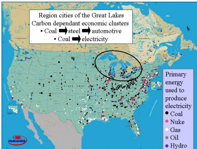
Figure 18 shows how electricity is produced in North America. The black, white, and grey are CO 2 based. The red is nuclear and the blue is the hydro. We use a lot of coal to produce electricity. Regardless of one's opinions, the Great Lakes region is basically a region of cities with very carbon-dependent economic clusters. We use coal, we use steel so we can have cars which, in turn, use petroleum. There is a huge issue on CO 2 management that will impact the Great Lakes region. Whether one likes it or not, it is there: Figure 18
