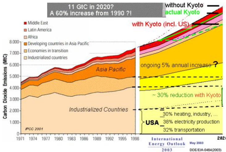
Figure 4 gives an idea of the picture from 1971 to 2020. People argue about greenhouse gas mitigation. Look at the graph without Kyoto, with Kyoto, and with Kyoto should the U.S. join. The main story is that most of the greenhouse gases will not come from North America. Rather, the big issue is that they will come from south-east Asia and China over the coming century. Figure 4
