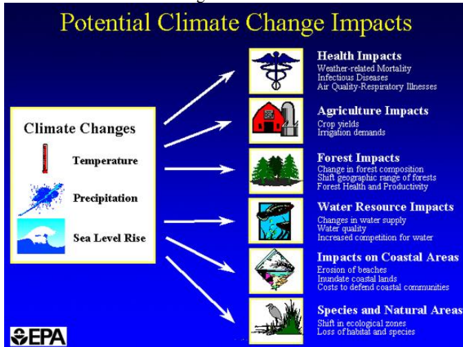
Figure 1. Potential Climate Change Impacts
